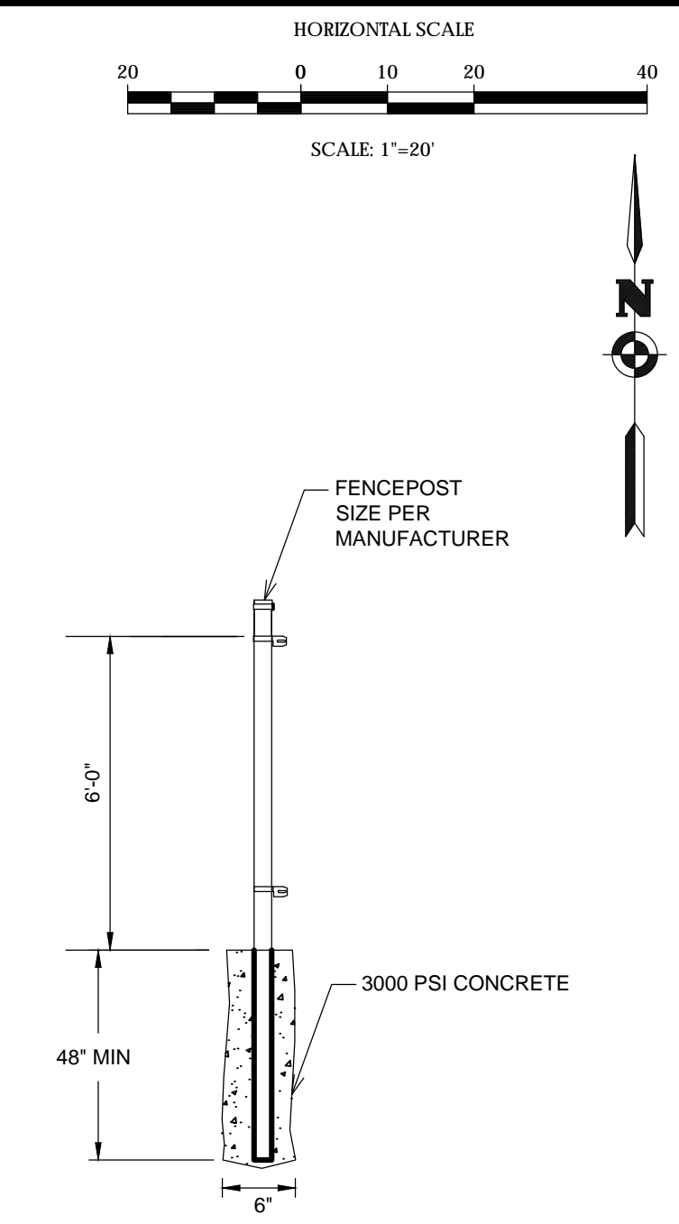
FENCE POST DETAIL
