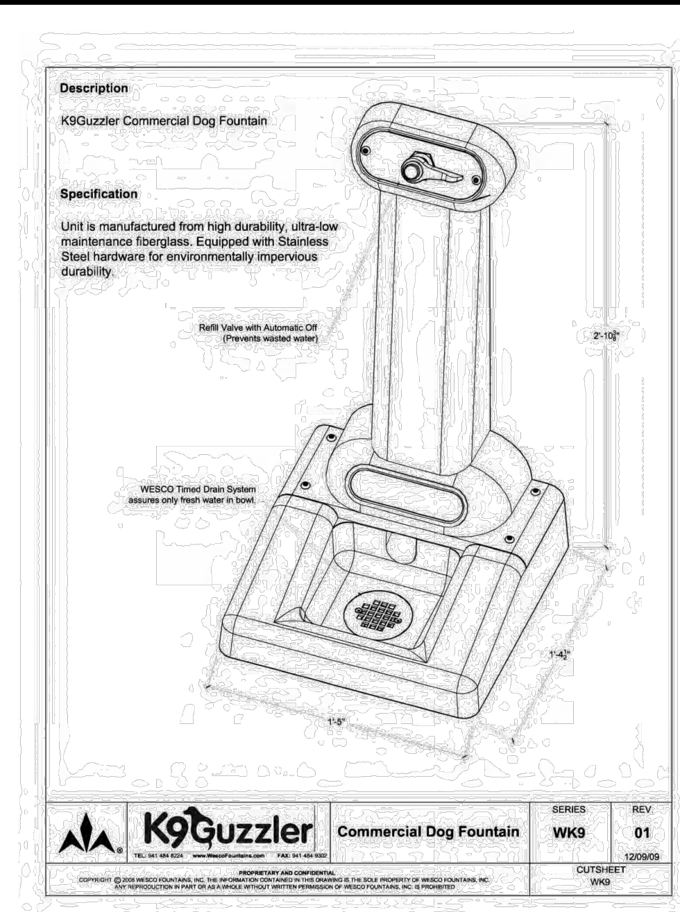
DOG DRINKING FOUNTAIN DETAIL
