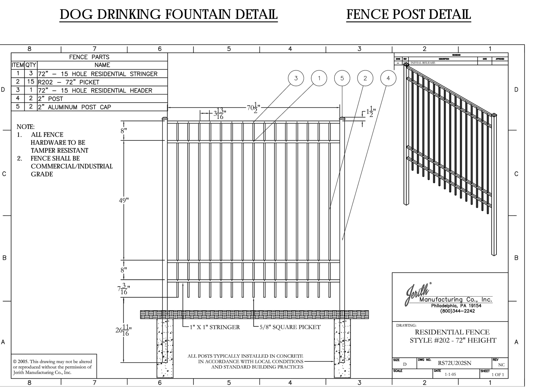
ALUMINUM FENCE PANEL DETAIL
